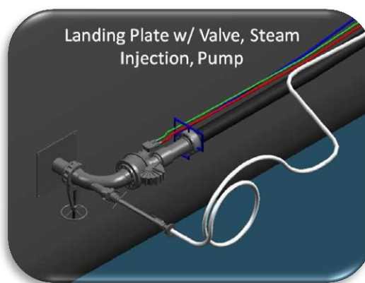
Figure 6 – SS LUCKENBACH Transfer Operations (1)
